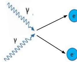
\gamma\gamma pair production
