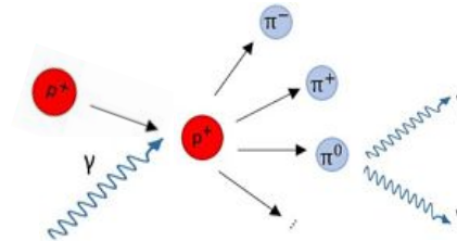
Photopion production
